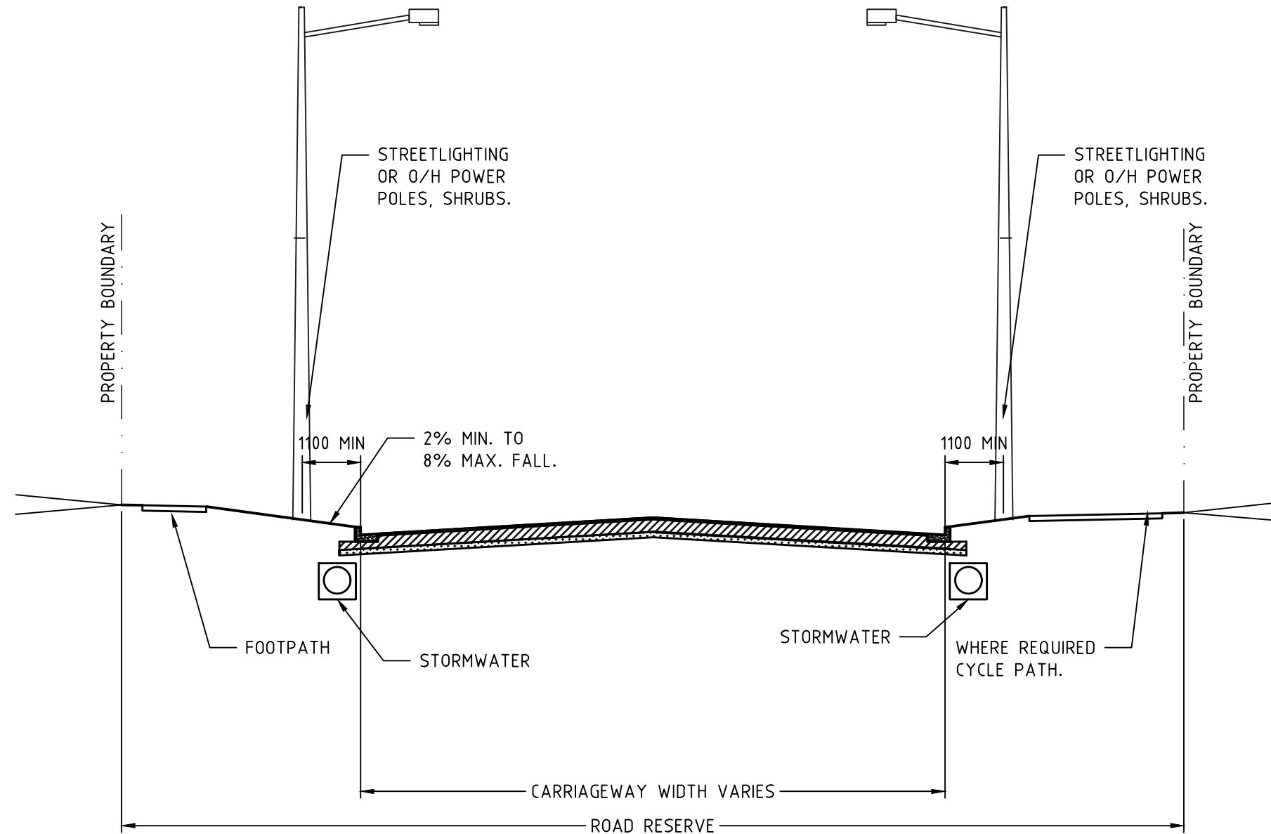
TYPICAL SERVICE SECTION NTS
